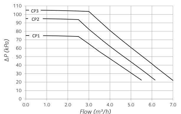
PUMP CHARACTERISTICS
