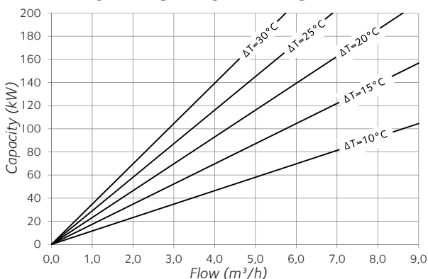
BOILER CAPACITY DIAGRAM
