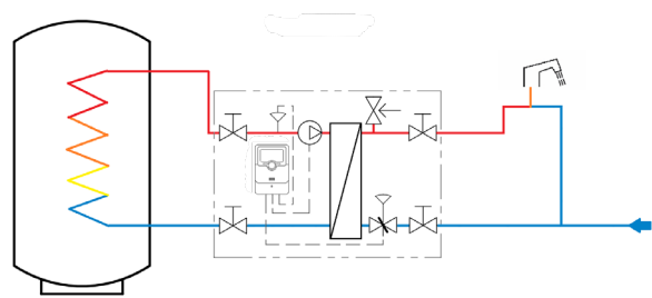
LK 250 TAPWATER UNIT P - WITH CONTROLLER
