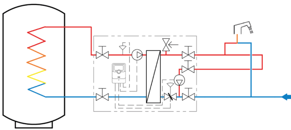
LK 250 TAPWATER UNIT P - WITH CONTROLLER AND HWC KIT (HOT WATER CIRCULATION)
