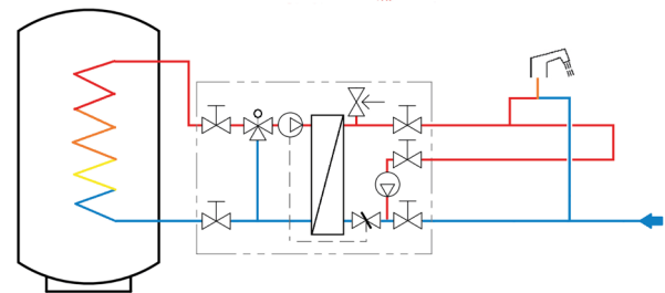
LK 250 TAPWATER UNIT - WITHOUT CONTROLLER WITH LK 551 AND HWC KIT (HOT WATER CIRCULATION)
