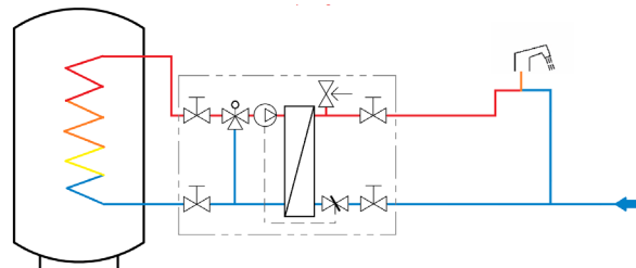
LK 250 TAPWATER UNIT - WITHOUT CONTROLLER
